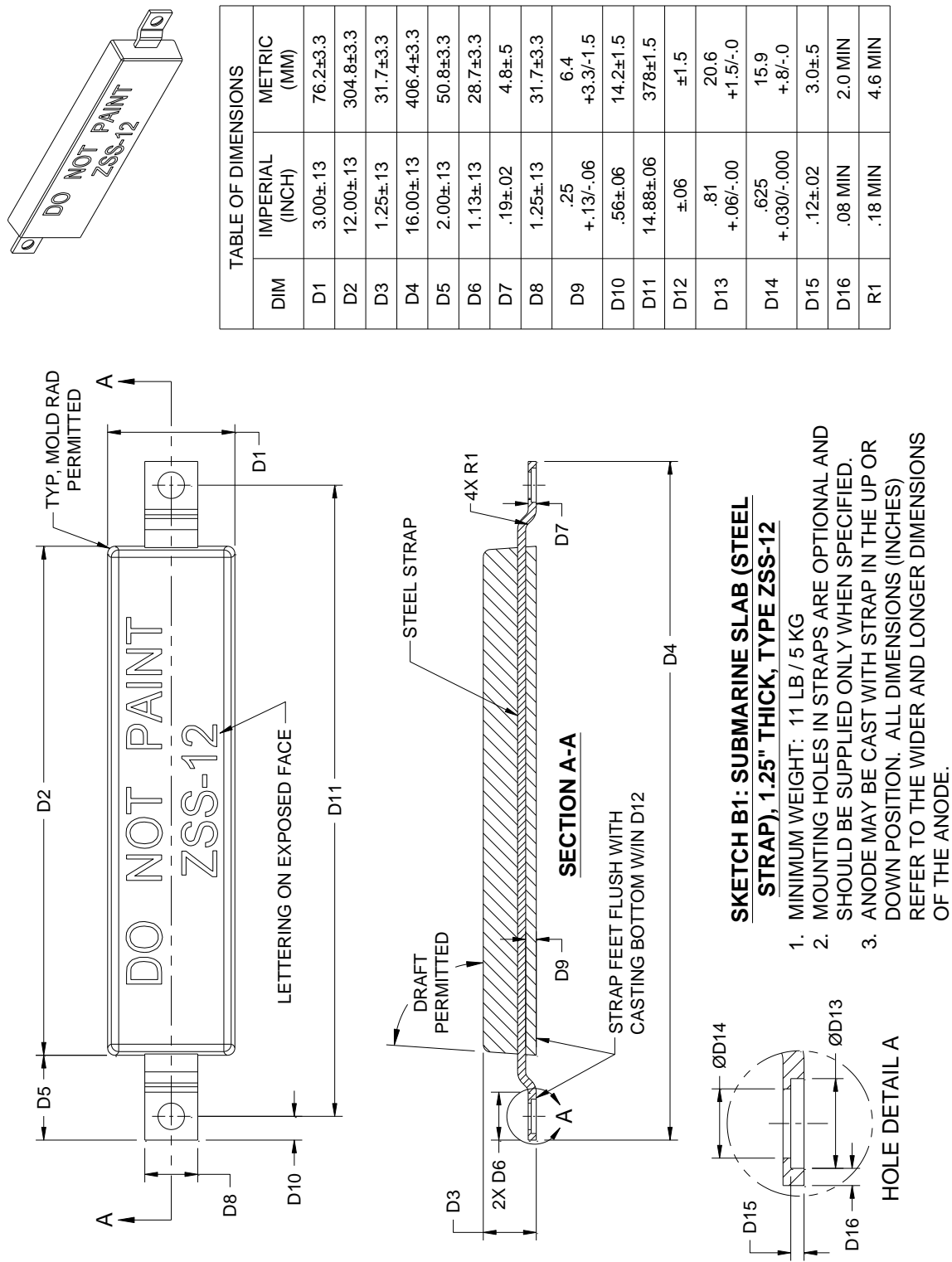
FIGURE 4. Zinc, submarine slab (steel strap), type ZSS-12.
