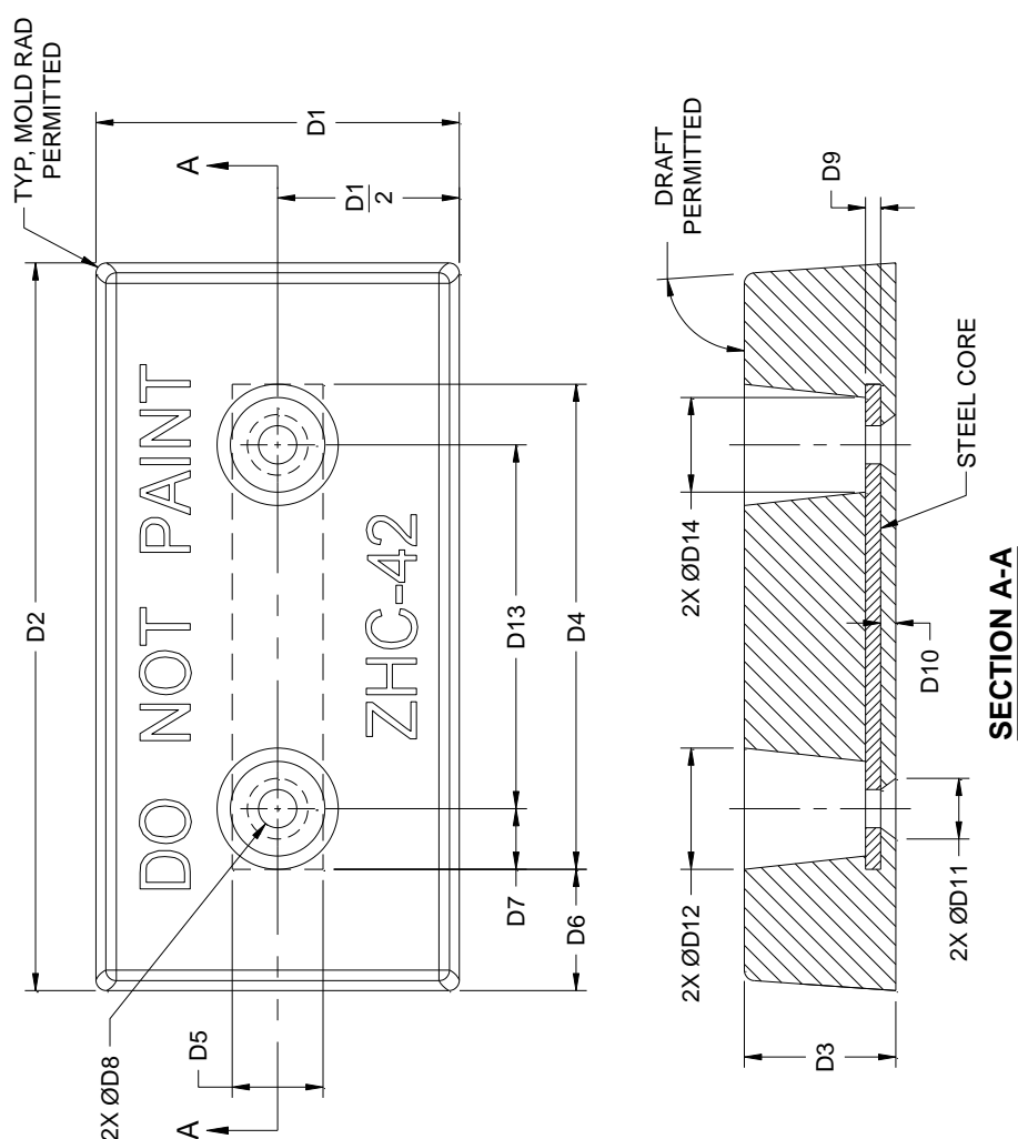
FIGURE 10. Zinc, hull slab (steel core), type ZHC-42.
