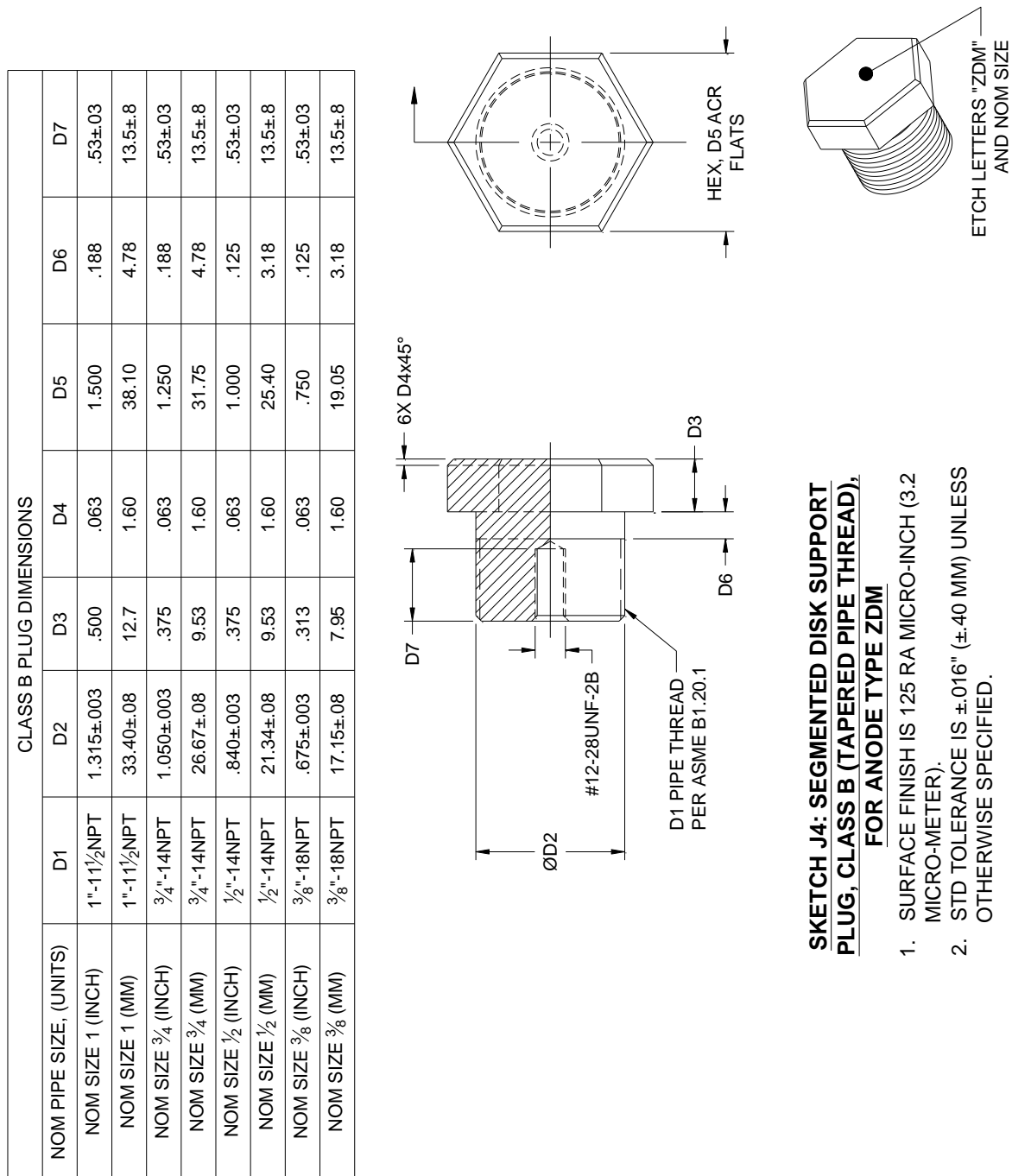
FIGURE 27. Zinc, segmented disk support plug, class B (tapered pipe thread), type ZDM.
